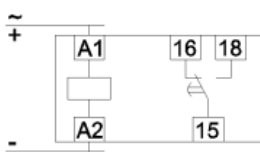
NTE8-C (4 wires) wiring diagram
