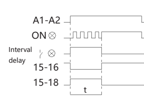
type D delay time sequence chart
