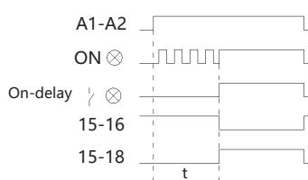
type Di delay time sequence chart
