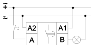
NTE8-C (3 wires) wiring diagram
