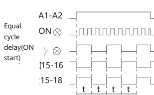
type Di delay time sequence chart
