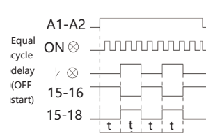
type D delay time sequence chart
