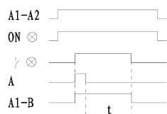
NTE8-Y time sequence chart
