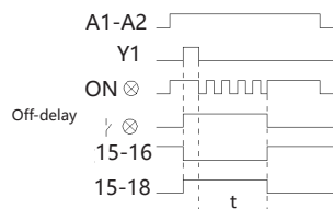
type B delay time sequence chart
