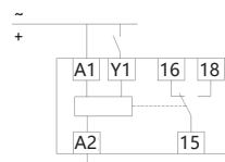
NTE8-M2 wiring diagram
