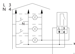
NTE8-C (3 wires) wiring diagram
