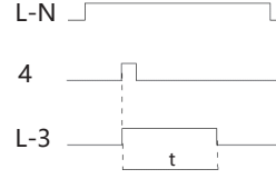
type H delay time sequence chart
