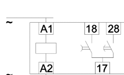
NTE8-Y wiring diagram
