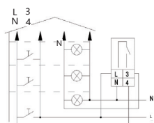
NTE8-C (4 wires) wiring diagram
