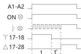
NTE8-Y time sequence chart
