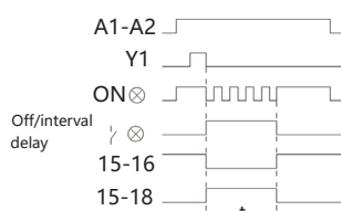
type W delay time sequence chart
